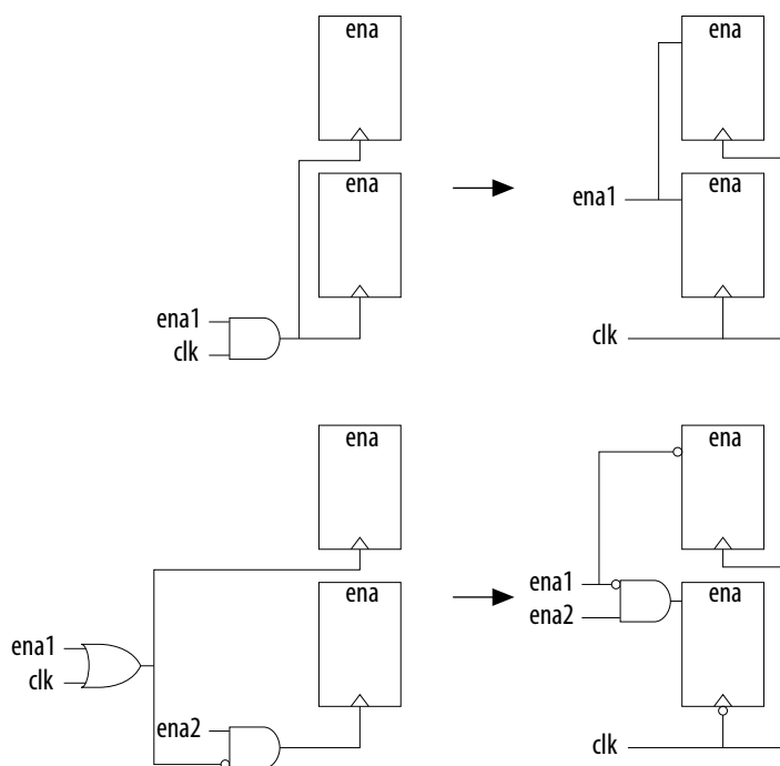
Figure 35. Example Gated Clock Conversion
