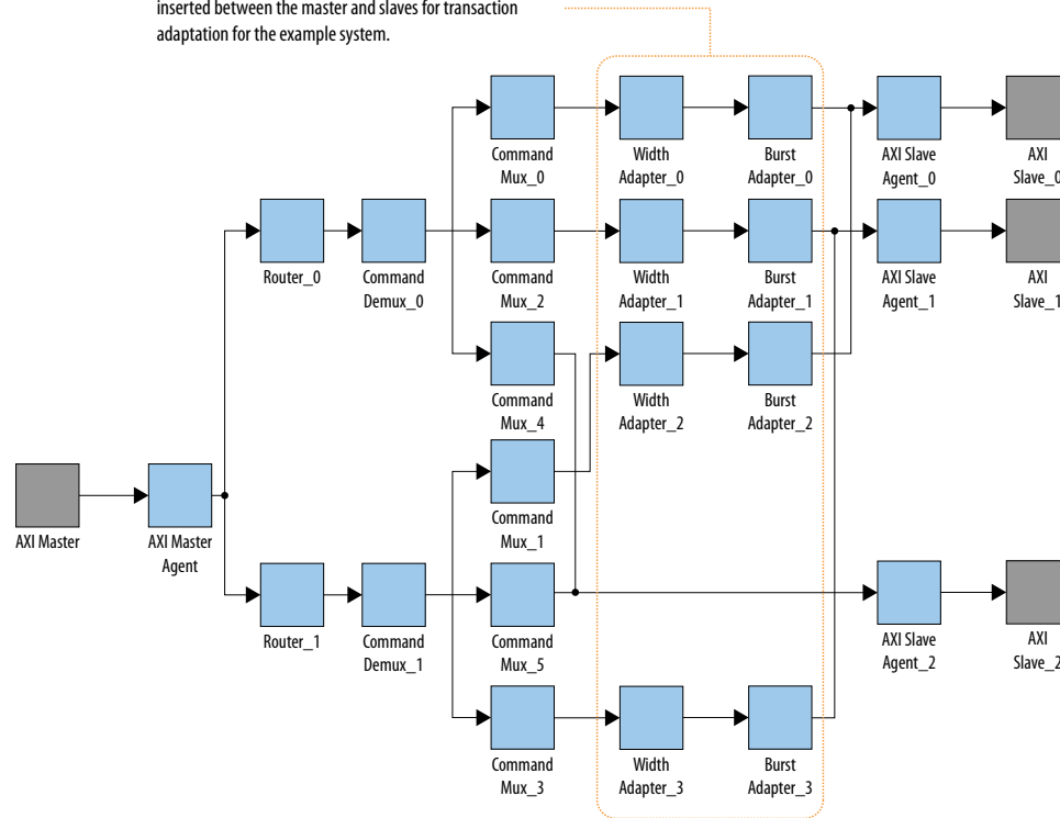
Figure 118. AXI System Without a Bridge
