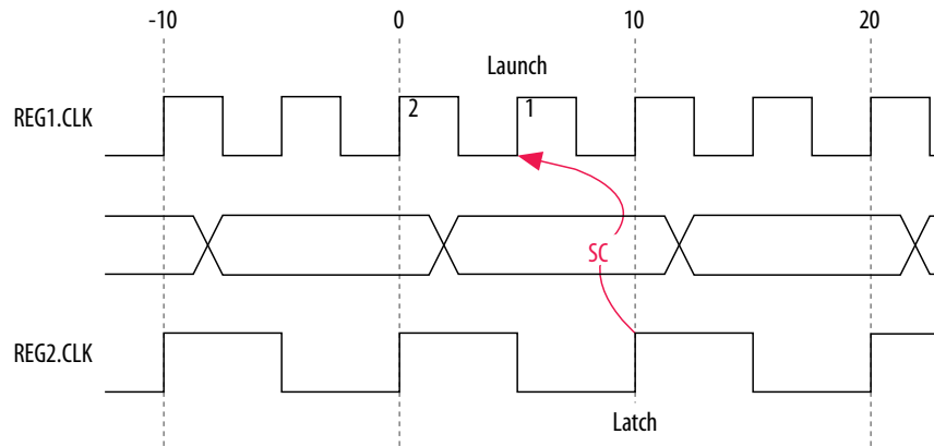
Figure 100. Setup Check Calculation
