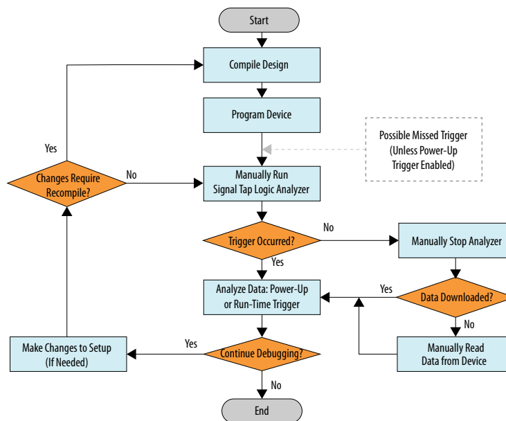
Figure 88. Power-Up and Runtime Trigger Events Flowchart
