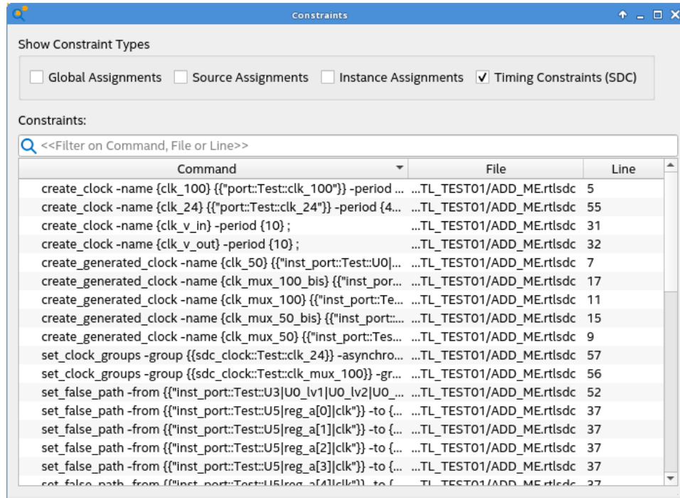
Figure 66. Constraints Viewer
