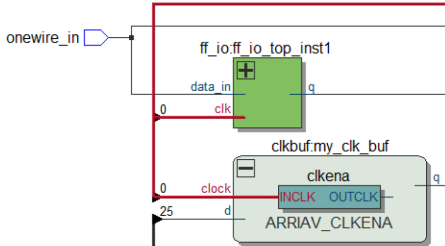
Figure 15. Show Connectivity Details
