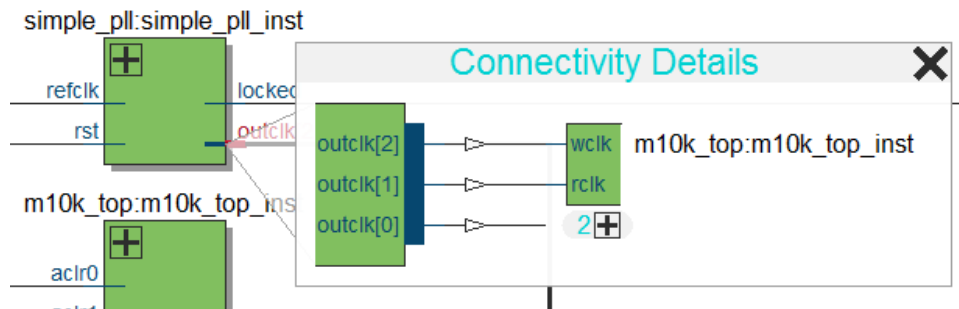
Figure 15. Show Connectivity Details
