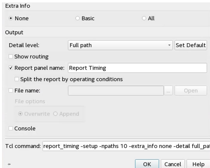
Figure 39. Report Timing Dialog Box (Bottom Section)
